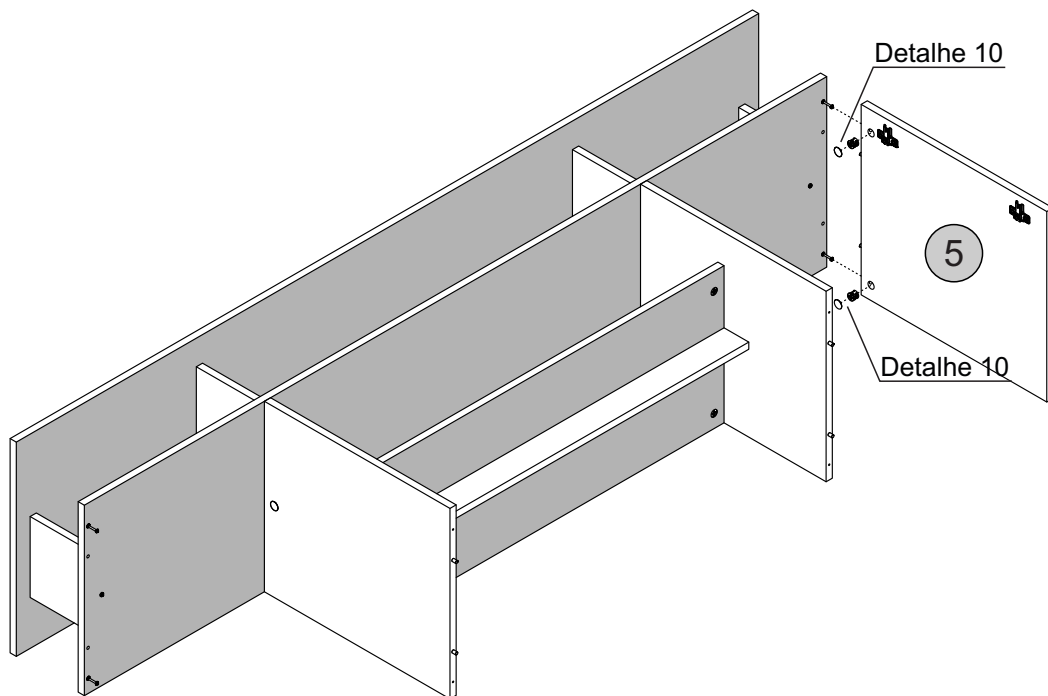
Detalhe 10 Detalle/Detail
