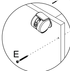
Detalhe 16 Detalle/Detail
