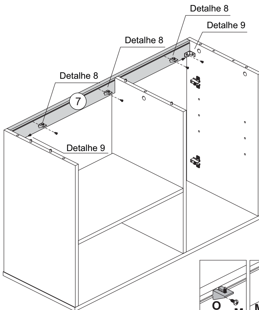
Detalhe 8 Detalle/Detail
