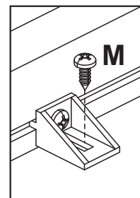
Detalhe 10 Detalle/Detail
